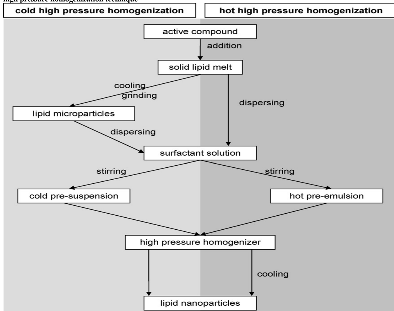
Figure 3. Production process of lipid nanoparticles using cold (light gray background) and hot (dark gray background) high pressure homogenization technique
